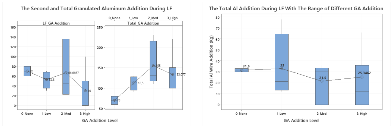
Figure 7: The granulated and wire aluminum additions. Left: Total and second batch GA additions with different range of primary GA addition level, Right: Aluminum wire additions with different range of primary GA addition level
