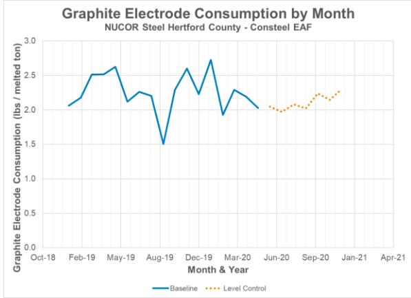
Figure 13: Plot of monthly electrode consumption at the Consteel EAF during the baseline analysis period (blue, solid line) and after implementing level control (orange, dotted line). NOTE: instances of electrode breaks were removed so as not to contaminate the analysis.
